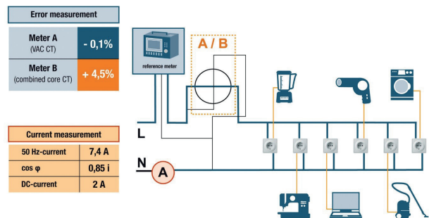
Fig. 8: Measurement example for a realistic \cos \varphi in a typical household
